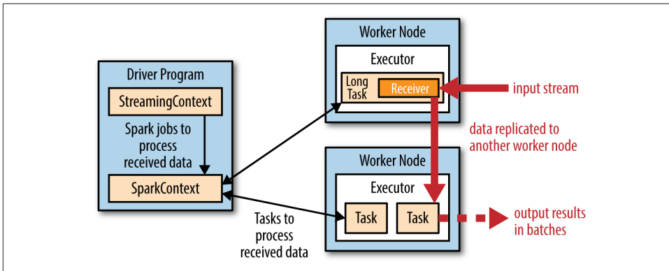
Figure 10-5. Execution of Spark Streaming within Spark's components
