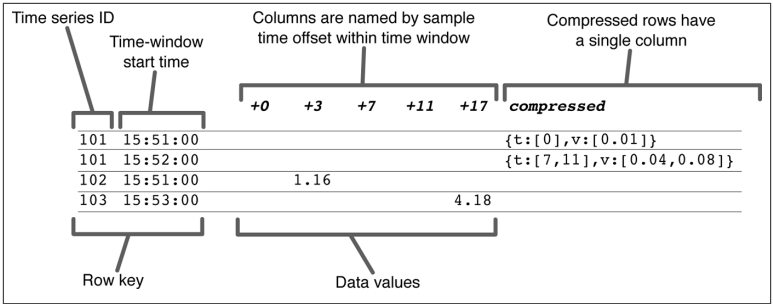
Figure 3-4. In the hybrid design, rows can be stored as a single data structure (blob). Note that the actual compressed data would likely be in a binary, compressed format. The compressed data are shown here in JSON format for ease of understanding.
