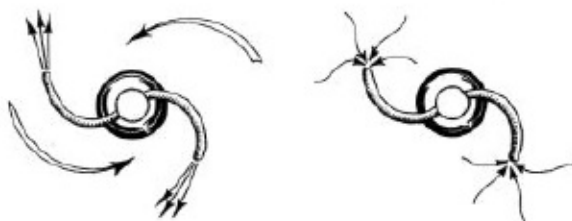
The mystery of the lawn sprinkler. When it sprays water, it spins counterclockwise. But what happens when it is made to suck water in?
