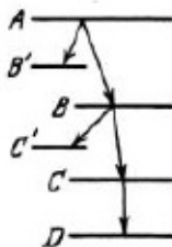
The “quantum jump” visualized as a sort of ladder.
