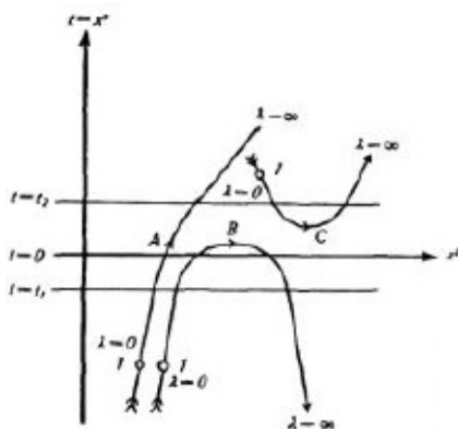
A diagram from a little-known 1941 paper of Ernst Stückelberg, showing aversion of time reversal in particle trajectories.
