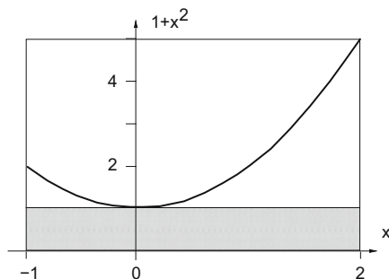
Fig. 6.7 The area below the graph of x^2 + 1 is between the areas of the smaller and larger rectangles. The height of the small rectangle is 1. The height of the large rectangle is 5
