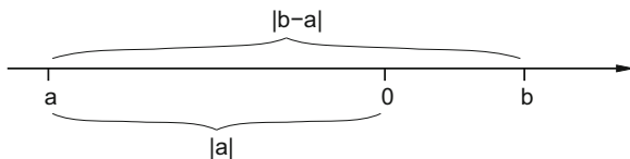
Fig. 1.3 Distances are measured using absolute value
