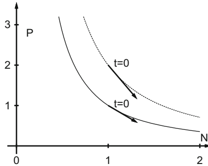
Fig. 10.17 The (N, P) -plane in a case of no predation, \frac{dN}{dt} = 2N , \frac{dP}{dt} = -3P . Two time histories are shown, one starting from (N_0, P_0) = (1, 1) and the other from (N_0, P_0) = (1, 2) . See Example 10.6
