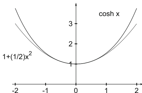
Fig. 3.32 The graphs of \cosh x and 1 + \frac{1}{2}x^2
