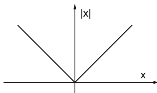
Fig. 3.5 The absolute value function is continuous, but it is not differentiable at 0. See Examples 3.6 and 3.8
