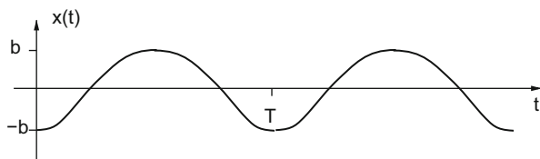
Fig. 10.6 The motion repeats with period T
