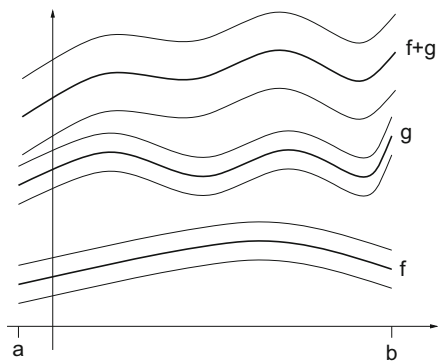
Fig. 2.39 Functions f_n are within \varepsilon of f for n > N_1 , and the g_n are within \varepsilon of g for n > N_2 . The sums f_n + g_n are then within 2\varepsilon of f + g for n larger than both N_1 and N_2
