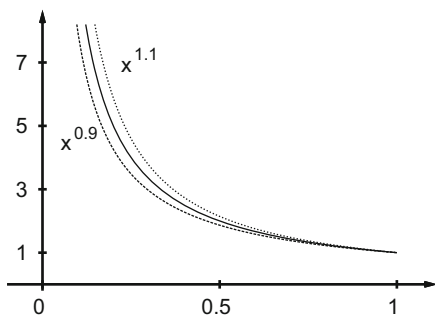
Fig. 7.9 The graphs of \frac{1}{x^p} for p = 0.9, 1 , and 1.1 , for Example 7.29. As h \rightarrow 0 , the area between [h, 1] and the graph converges if p < 1 and diverges if p \geq 1
