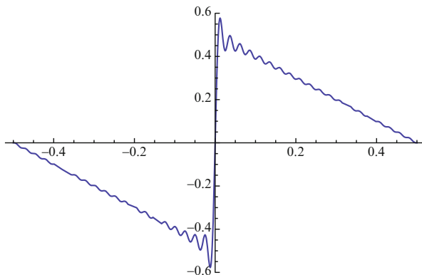
Fig. 3.3 The partial sums (h * D_{40})(t) showing the overshoot of approximately 9% of the jump of h at zero.
