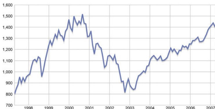
Fig. 17.4 Daily closing values of the S&P 500 index, April 1997 to April 2007. (Source: New York Stock Exchange)
