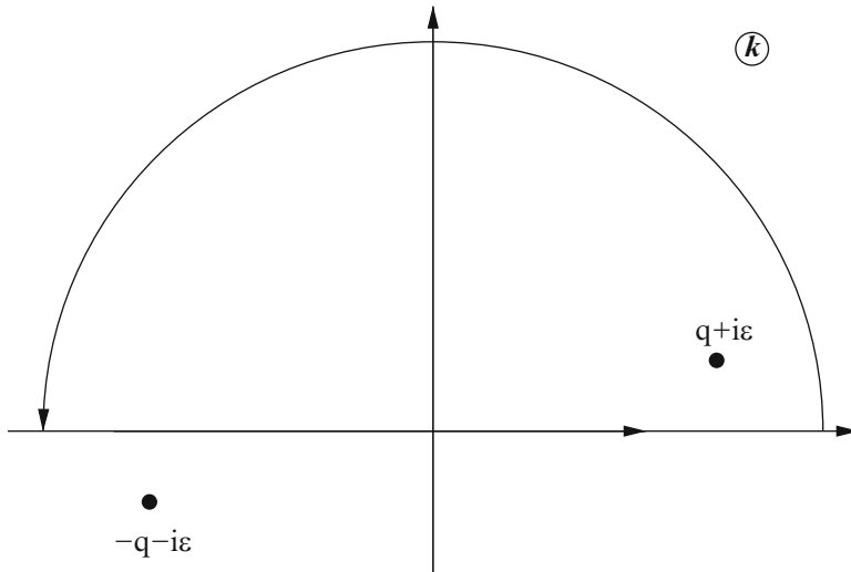
Fig. 11.1 Location of the poles and integration contour in the complex k plane. Here q \equiv \sqrt{2mE}/\hbar
