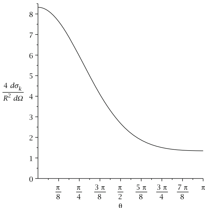
Fig. 11.4 The differential scattering cross section d\sigma_k/d\Omega of a hard sphere of radius R normalized to the classical differential scattering cross section (d\sigma_k/d\Omega)_{\text{classical}} = R^2/4 for kR = 1
