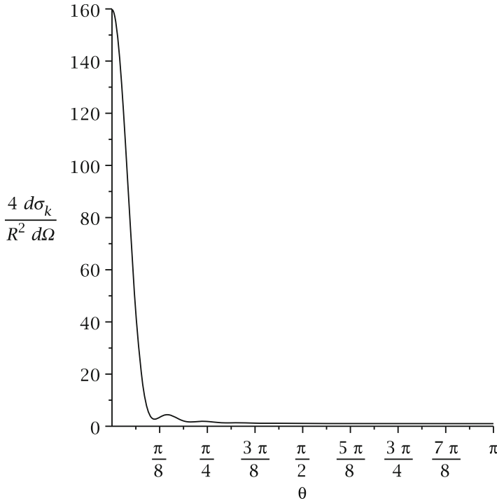
Fig. 11.5 The differential scattering cross section d\sigma_k/d\Omega of a hard sphere of radius R normalized to the classical differential scattering cross section (d\sigma_k/d\Omega)_{\text{classical}} = R^2/4 for kR = 10
