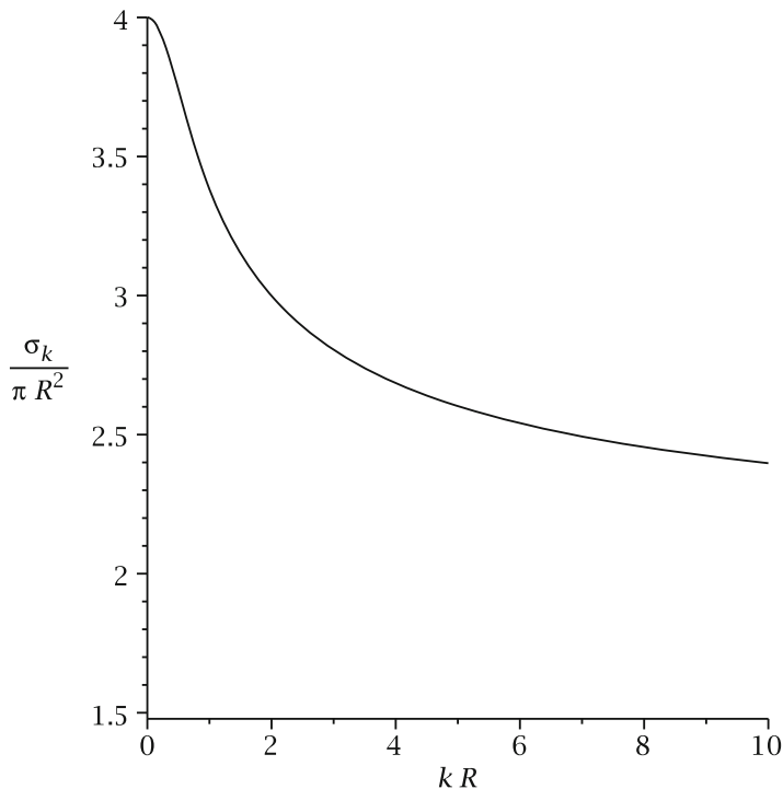
Fig. 11.3 The scattering cross section of a hard sphere normalized to the classical scattering cross section \sigma_{\text{classical}} = \pi R^2
