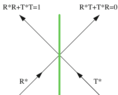
Fig. K.1 Amplitudes at the beam splitter, laterally reversed on the right side
