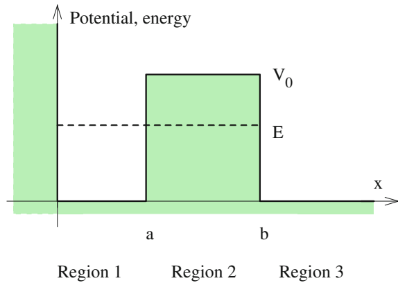
Fig. 15.13 The potential of (15.93)
