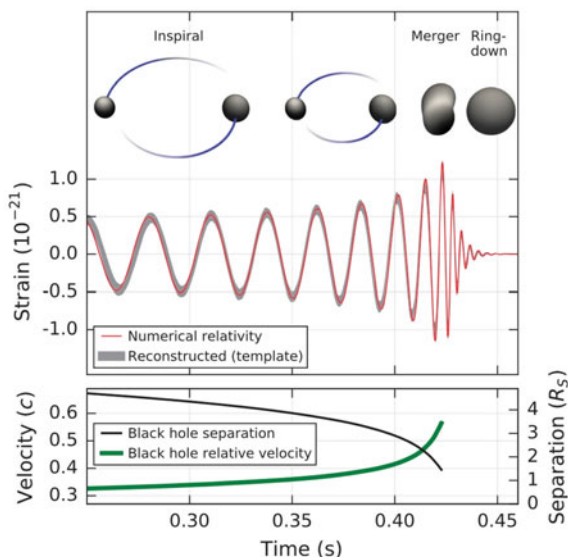
Fig. 12.3 Temporal evolution of the strain, of the black hole separation, and of the black hole relative velocity in the event GW150914 (see Sect. 12.7 for the definition of strain). From [1] under the terms of the Creative Commons Attribution 3.0 License
